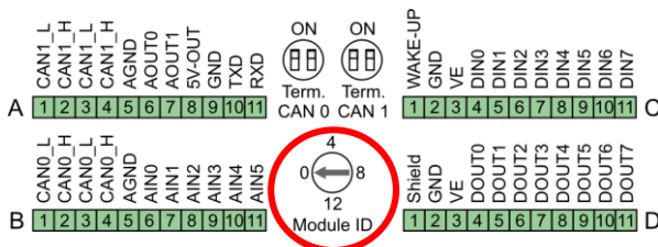
Rotary switch for the module ID (industrial model)
