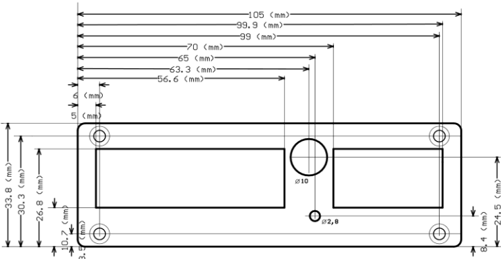
Front of the automotive model
