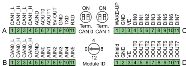
Connector pin assignment of the industrial model
