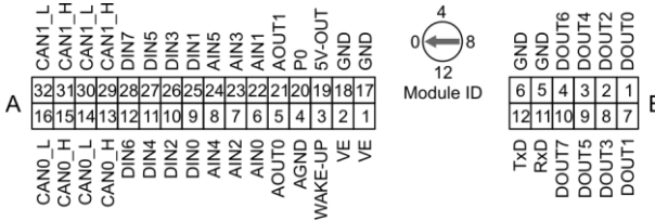
Connector pin assignment of the automotive model
