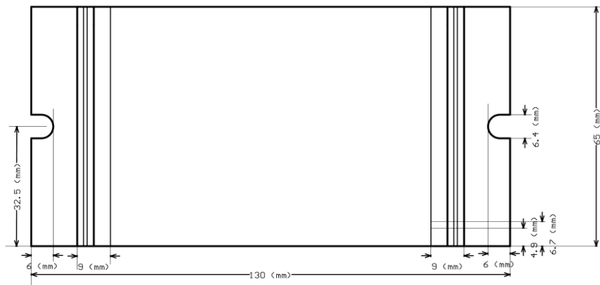
Top view of the bottom plate
