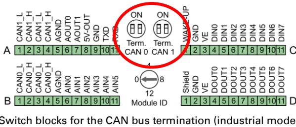
Switch blocks for the CAN bus termination (industrial model)
