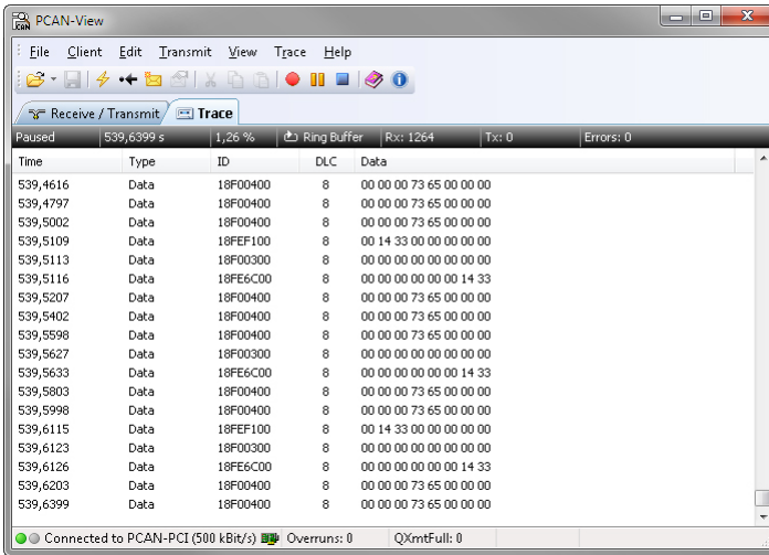
Figure 8: Trace Tab
