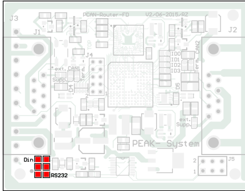
Position of the solder fields for switching between RS-232 and Din (pre-equipped with 0-Ohm resistors)
